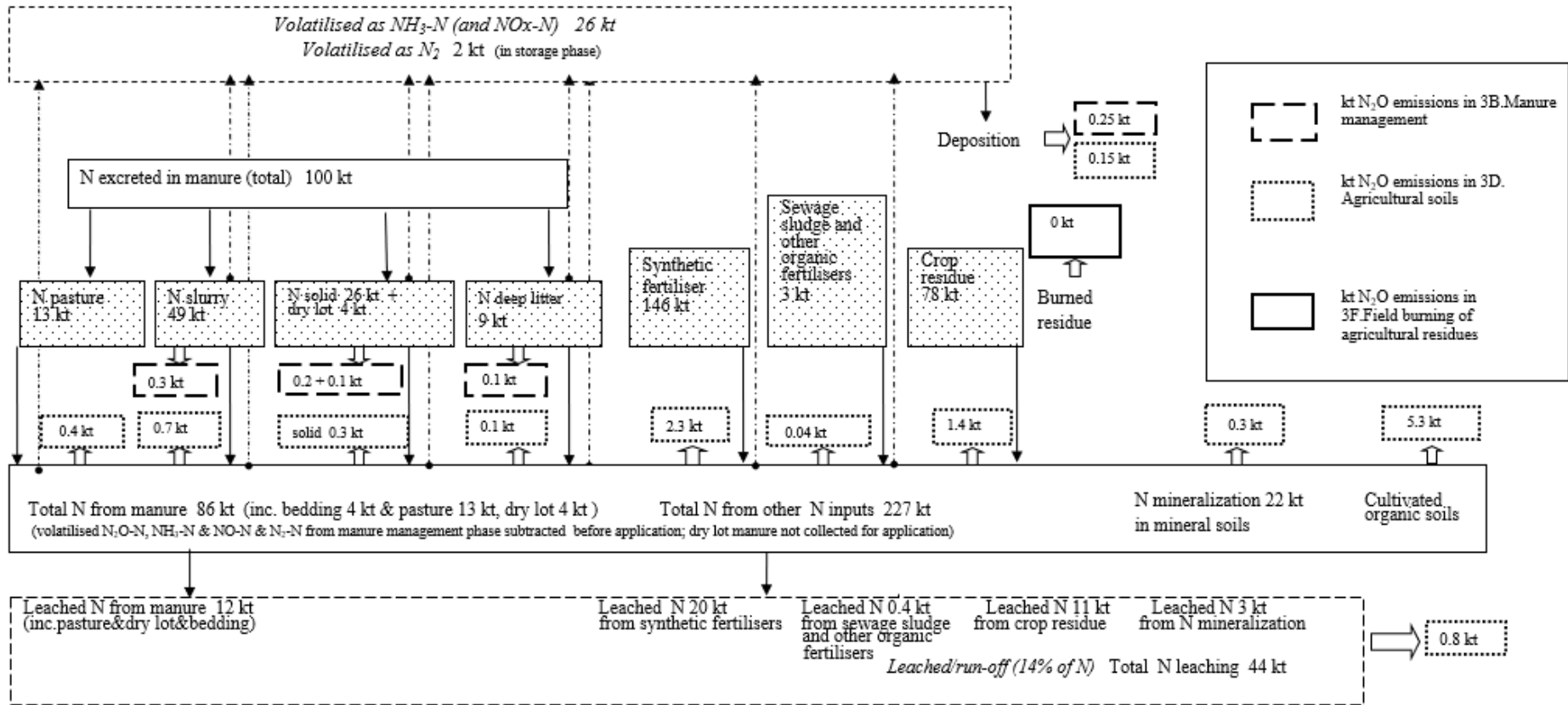
Figure 5.1-4 Nitrogen flows and nitrous oxide emissions in the Agriculture sector in 2021. Thin arrows denote N flows, of which dashed arrows show N volatilisation as ammonia, nitric oxide and dinitrogen. Bulk arrows denote N 2 O emissions. Nitrogen flows are in kt N year -1 and emissions (dotted line) in kt N 2 O year -1 . Figures are rounded, subtotals and totals calculated from unrounded values.
