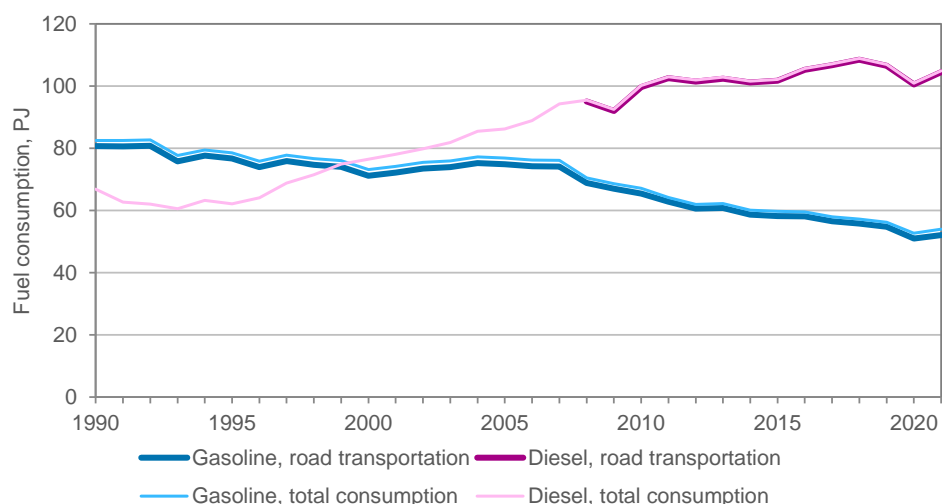
Figure 3.2-12 Consumption of diesel oil and gasoline (including bioshares) in road transportation in 1970 to 2020 (Energy Statistics, Statistics Finland).
