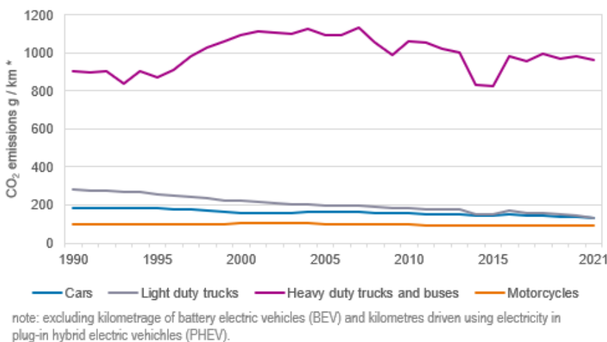
Figure 3.2-11 CO 2 emissions per kilometre (LIISA Model)
