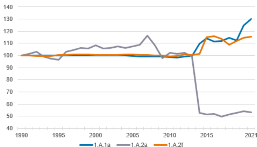
Figure 3.2-3 Indexed CO 2 implied emissions factor of solid fuels
