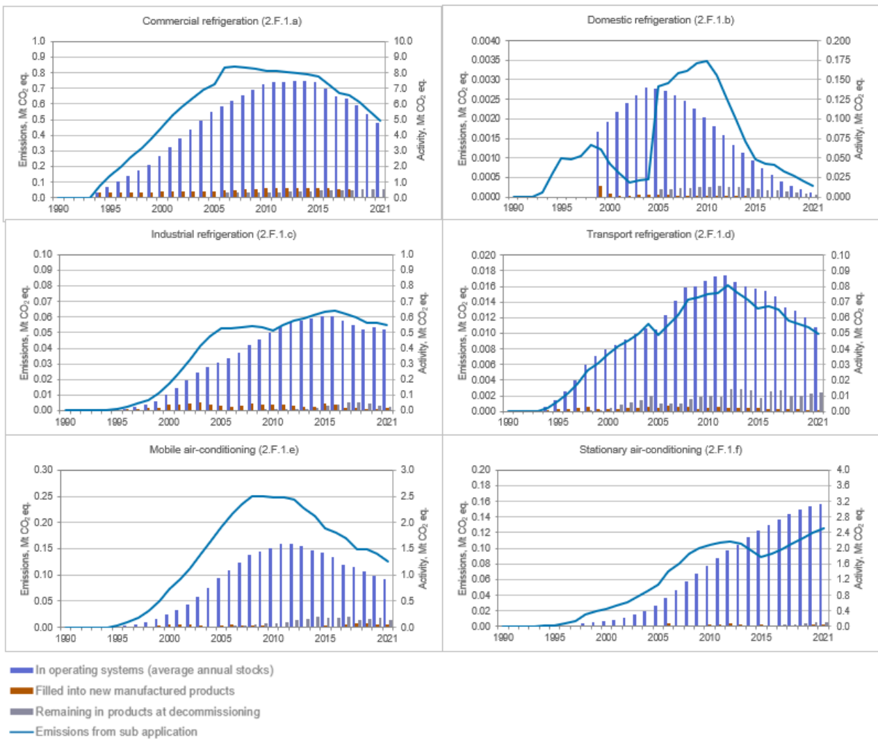
Figure 4.7-3 Total greenhouse gas emission and amounts of gas in operating systems, filled into new manufactured products and remaining in products at decommissioning of six subcategories of the Refrigeration and air conditioning equipment (Mt CO 2 eq.)
