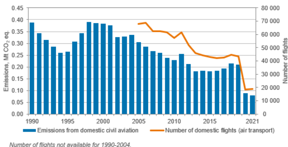
Figure 3.2-8 Emissions from domestic civil aviation (Mt CO 2 eq.)
