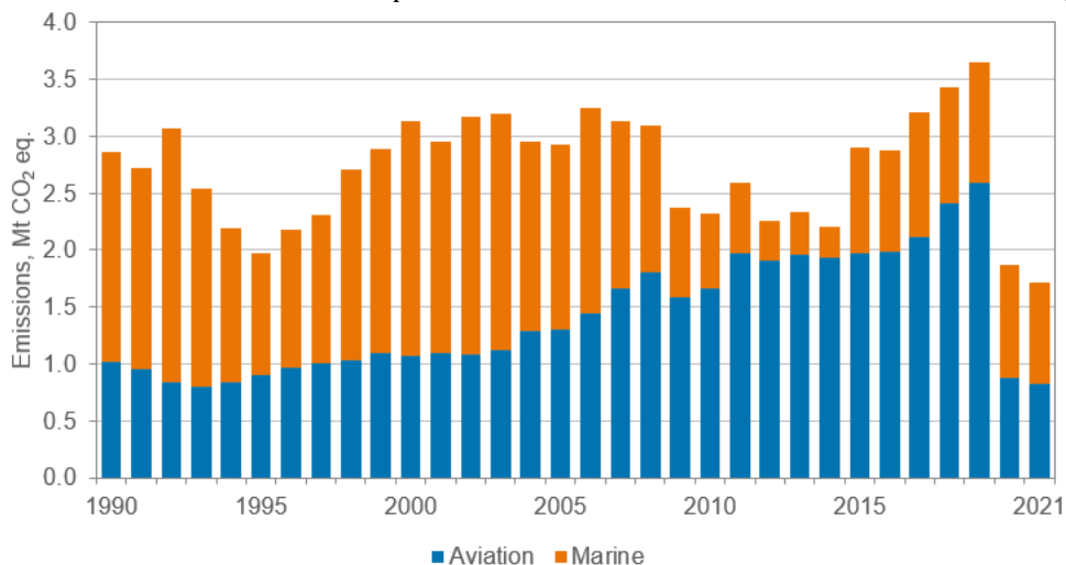
Figure 3.2-2 Emissions from international bunker, Mt CO 2 eq.
